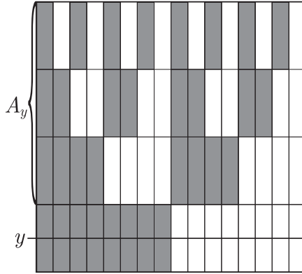
FIGURE 8.1. A model for \varphi_4 on [0, 1] .
